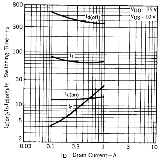
SWITCHING CHARACTERISTICS
